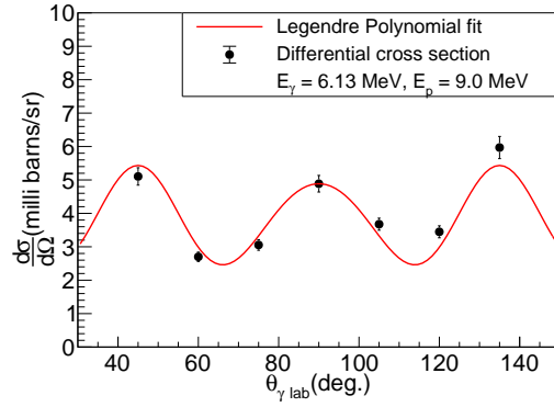
FIG. 2: Differential cross-section of 6.13 MeV \gamma -ray for various angles at 9 MeV energy of incident proton. Red line is the fit of Legendre polynomial series.
